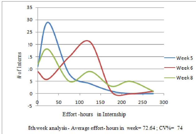
Fig. 3. Distribution of Effort Hours vs Number of Interns
